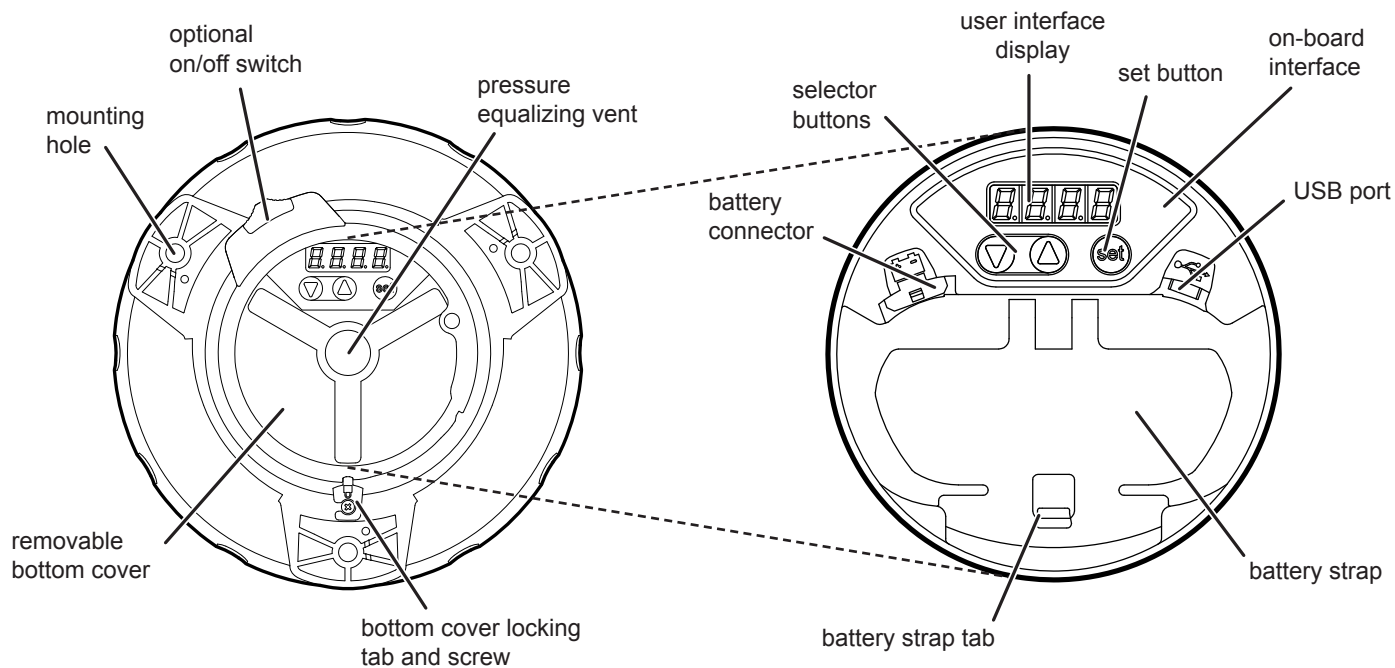
BOTTOM VIEW
